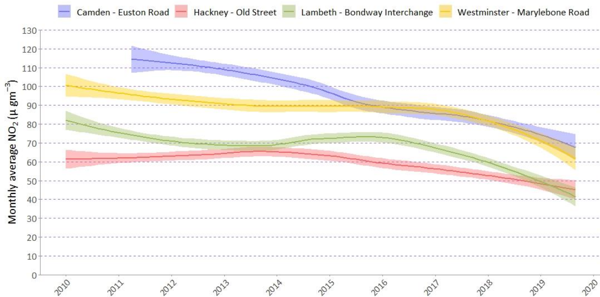
Figure 10.3 Trends in NO 2 on ULEZ boundary roads, 2010-2019.
