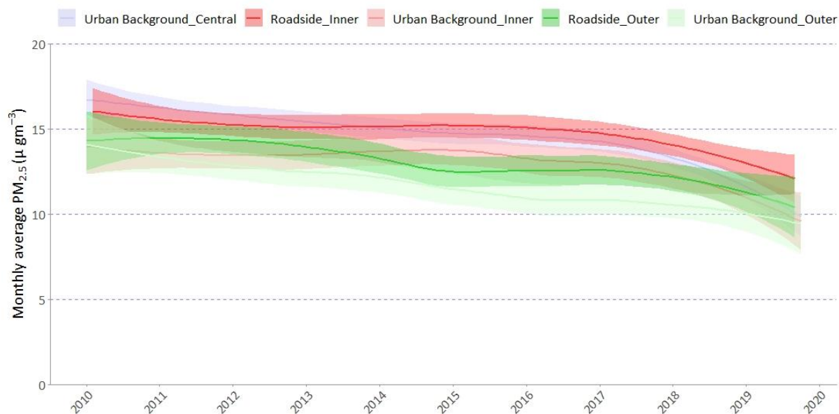
Figure 10.4 Trends in PM 2.5 in London, 2010-2019.
