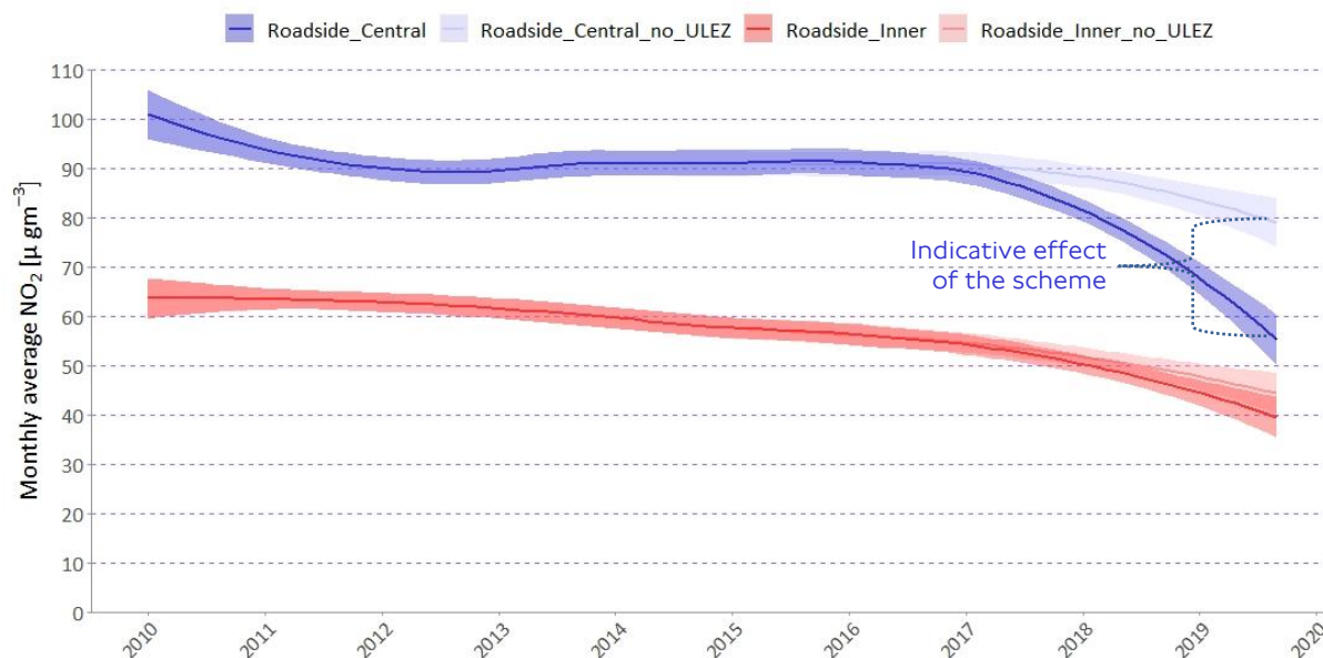
Figure 9 NO 2 concentrations for central and inner London, 2010-2020.
