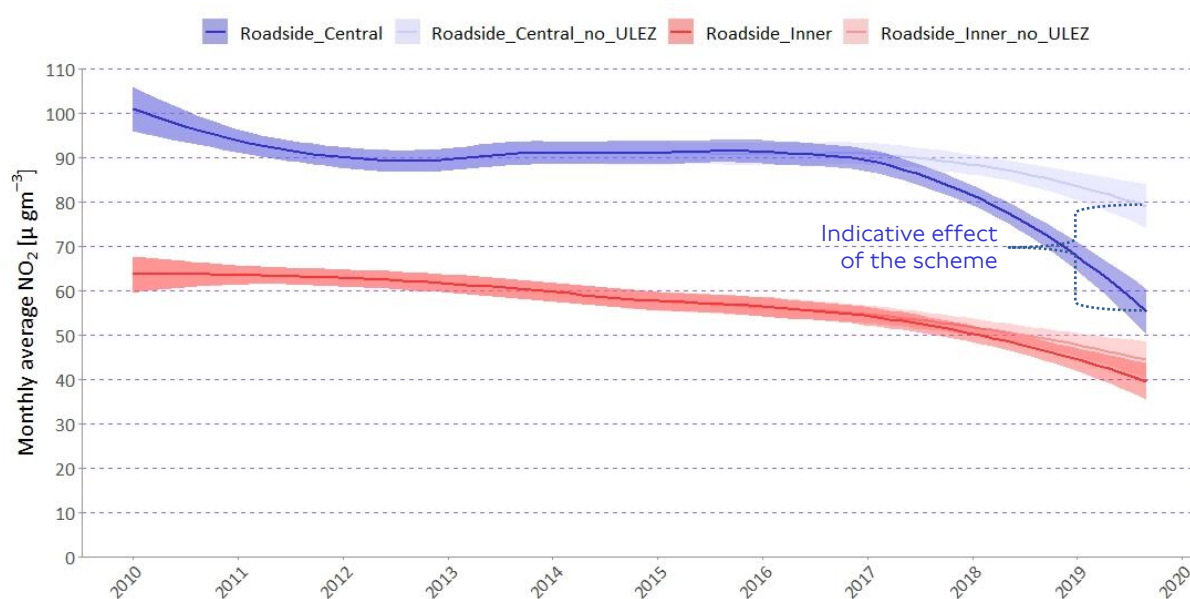
Figure 10.2 Comparison of 'business as usual' trends in NO 2 concentrations with observed concentrations in central and inner London, 2010–2019.
